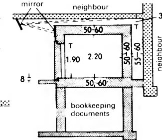
⑩ + ⑪ Strongroom surrounded by neighbouring walls
